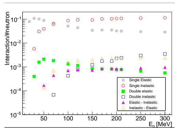
Figure 2: Number of interactions per primary neutron as a function of the neutrons initial kinetic energy.
