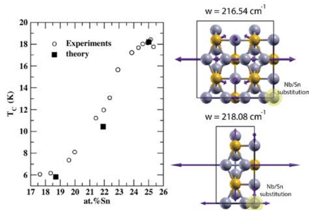
Figure 2: T c degradation of Nb (3-x) Sn (1+x) compounds and the surviving coupling phonon modes.
