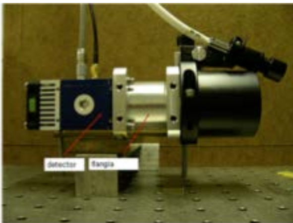
Figure 1: PTR compact device for measurements of gears.
