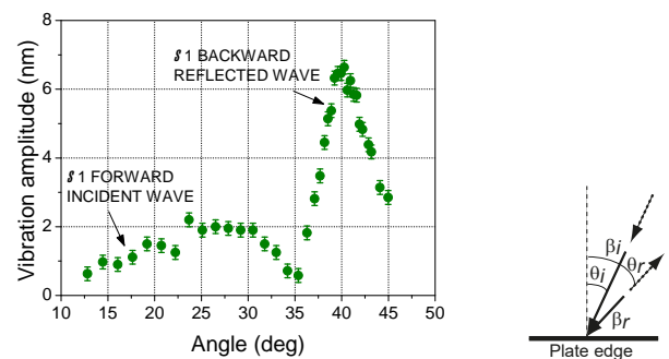
Figure 1: Profiles of the surface vibration amplitudes along a line parallel to the plate edge. On the right side, diagrams of the relative geometrical relationships: the solid vectors refer to wave vectors, the broken ones to energy propagation directions. S_1 Lamb forward mode incident on the plate edge at an angle \theta_i = +25^\circ is converted into S_1 Lamb backward mode and reflected at angle \theta_r = +35 \pm 2^\circ . Conversion from forward to backward mode causes the angle of reflection to be changed from the incident one and lying on the same side with respect to the normal (negative reflection).
