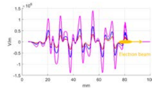
Figure 3: E_z behind the electron beam, after t = 0.29 ns from the cathode emission, for different beam total charges: 50 pC (red); 100 pC (blue); 200 pC (magenta).
