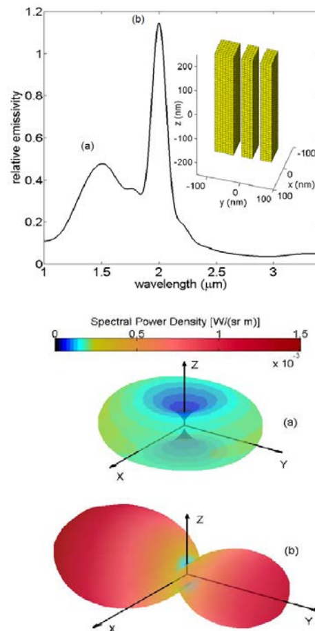
Figure 1: relative emissivity as a function of wavelength calculated for the coupled Au dipole nanoantennas sketched in the inset and described in reference [2]. The corresponding emission patterns of the two main peaks labelled (a) and (b) are depicted below.
