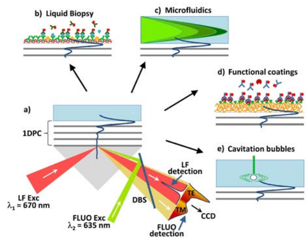
Figure 1: (a) Simplified sketch of the BSW based label-free and fluorescence sensing configuration. Applications: (b) specific probe antibodies bound at the surface capture biomarkers in human plasma, originating a label-free signal. Detection with a second labeled specific antibody permits to sense in the fluorescence mode; (c) BSW sense in label-free manner the liquid flow in proximity of a surface (100 nm); (d) the efficiency of functional coatings for human implants is tested by means of BSW; (e) pressure changes generated by a cavitation bubble in proximity of a surface is measured in a label-free manner.
