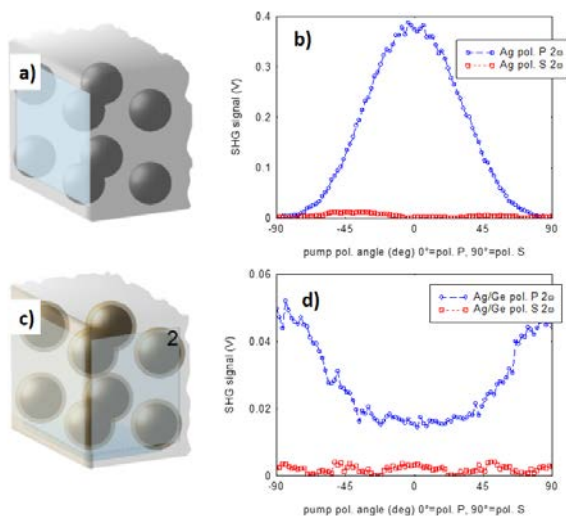
Figure 1: Figure 1: a) sketch of a polycrystalline silver film composed by crystal grains; b) SHG measurements on silver film as a function of input polarisation; c) sketch of a metasurface composed by silver grains surrounded by a Ge thin coating; d) SHG measurements on the Ag-Ge metasurface.
