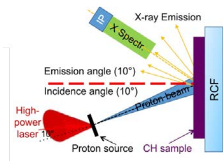
Figure 1: Experimental setup of laser-driven PIXE.
