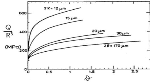
Figure 2: Torsional response of copper wires: the same normalized torque Q/R^3 produces a smaller twist \vartheta on wires of smaller radius R [Acta Metall. Mater. 42 475 (1994)].
