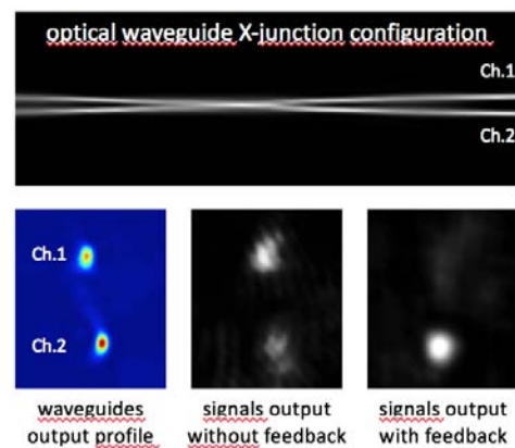
Figure 3: Simulation and experiment of an X-junction that can change performances according to an optical feedback injected in the network.
