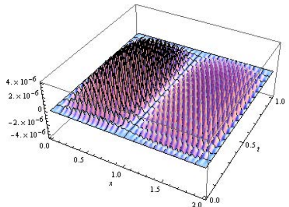
Figure 2: The error for \gamma = 0.25 and \Delta t = \Delta x = 0.03125 .
