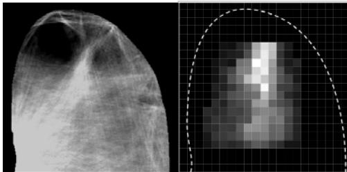
Figure 1: Theory and the experiment of biophotons emission and focusing by the seed-coat over the plumula of the embryo
