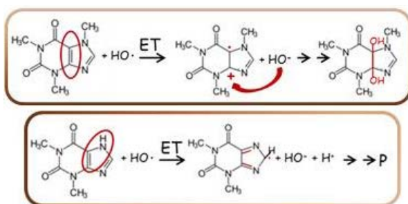
Figure 1: Oxidative mechanism of caffeine.
