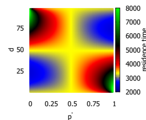
Figure 1: Residence time as a function of the position of the defect site d and the right jump probability p' .
