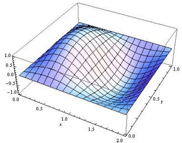
Figure 1: The numerical solution for \gamma = 0.25 and \Delta t = \Delta x = 0.03125 .
