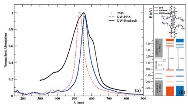
Figure 3: Theoretical and experimental BT2N absorption spectra.
