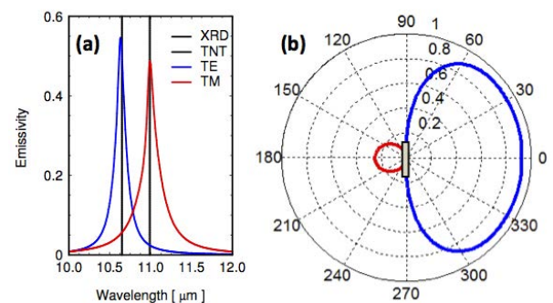
Figure 2: Spectral emissivity calculated for a system composed by oriented SiC inclusions into air matrix [3]. (b) polar plot of emissivity curve calculated at 10.48 micron, for a SiC layer 4 microns thick with graded air porosity [4].
