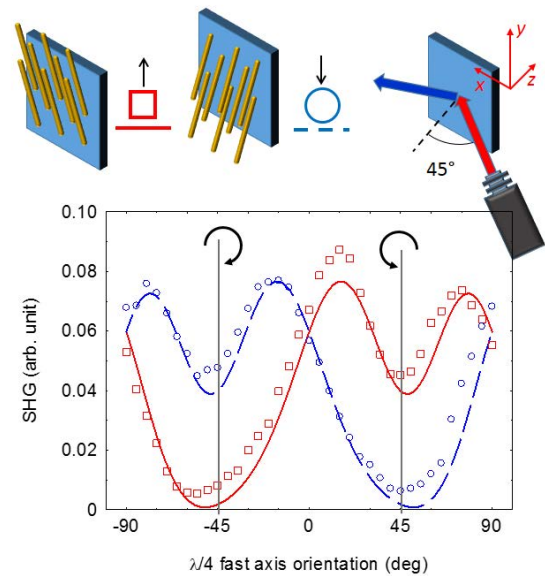
Figure 2: Figure 2: SHG measurements of the extrinsic chirality in a sample formed by gold tiled nanowires.
