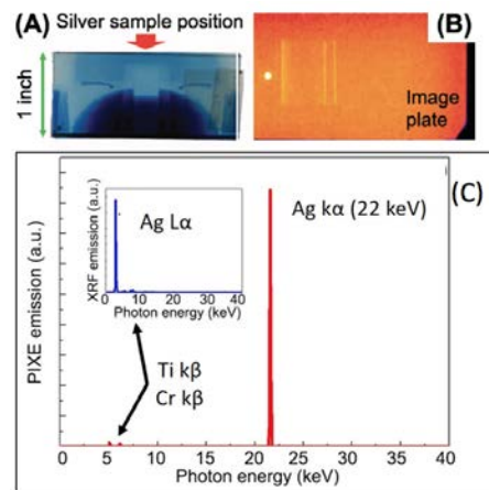
Figure 2: (A) Silver sample mounted on an RCF. (B) IP detecting the emitted X-rays. (C) Retrieved PIXE spectrum and RXF analysis (as reference) of the Ag sample.
