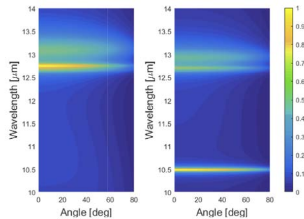
Figure 1: Emissivity spectra calculated for TE polarized fields as functions of wavelength and incidence angle for (a) a single SiC layer and (b) a SiC layer with 20% oriented air inclusions. SiC thickness is 1 micron, onto a Si substrate.
