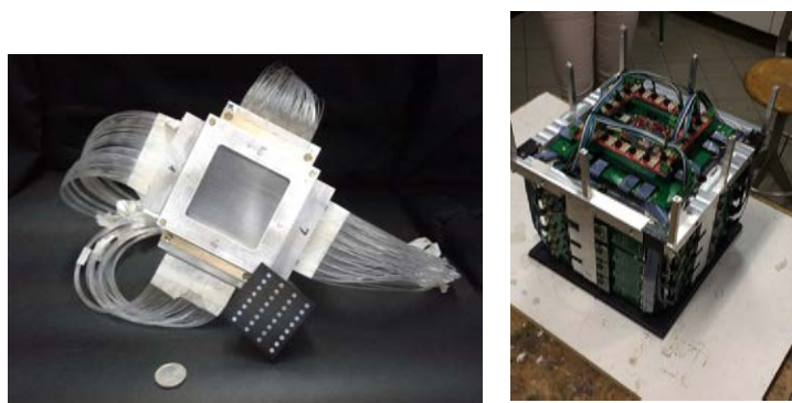
Figure 2: (Left) Plastic scintillator detector optimised for ToF measurements. The readout is performed using fibres. (Right) Dose Profiler detector: a charged particles tracker optimised for the monitoring of Particle Therapy treatments performed using carbon ions.
