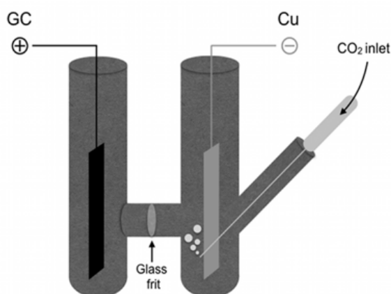
Figure 1: Electrochemical cell for CO 2 reduction.
