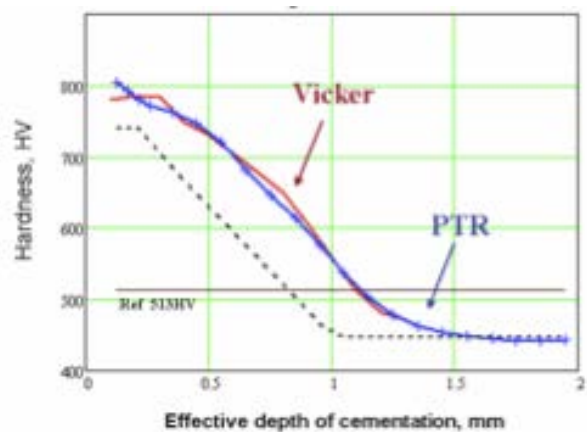
Figure 2: Hardened depth profiles in AISI9310 steels. Comparison between standard Vicker test (red line) and PTR NDT (blue line)
