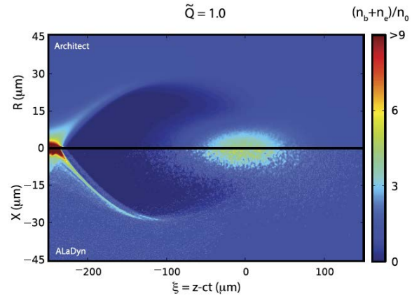
Figure 2: Cylindrical plasma channel for PWBA. A bunch is moving from left to right. The green-yellow spot on the axis around \xi = 0 is the driver bunch; on its left we observe a depleted bubble . The figure shows maps of electron density computed with the hybrid code Architect (top panel) and fully kinetic PIC code Aladyn (bottom panel) in a weakly nonlinear regime, confirming the adequacy of the much faster hybrid code.
