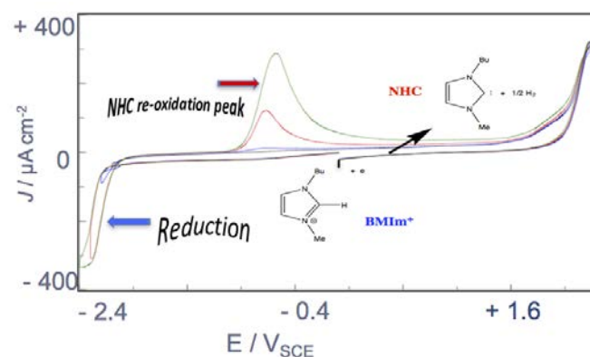
Figure 2: Cyclic voltammetry of \text{BMIm-BF}_4 .
