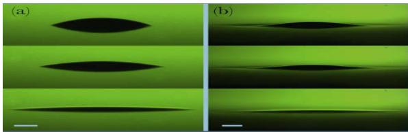
Figure 1: Silicone oil droplets spreading on thin films of the same oil with different thicknesses [PRL 109 154501 (2012)].
