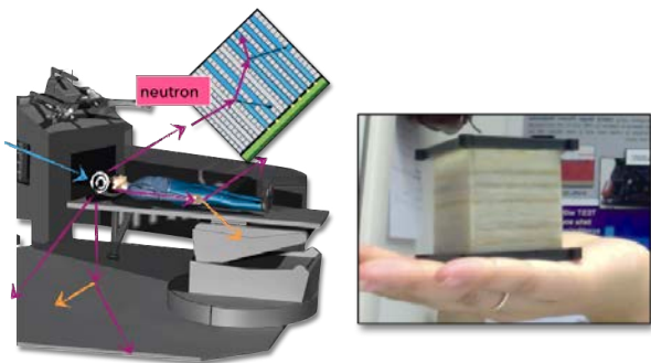
Figure 1: Left. Schematic representation of the secondary neutrons produced in PT interacting in the treatment room. The MONDO detector is shown on top of the scratch. Right. First MONDO prototype.
