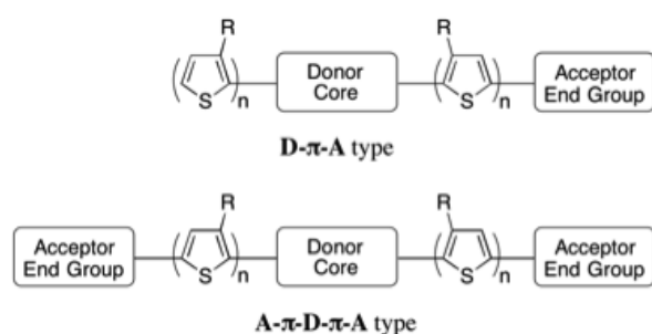
Figure 1: D- \pi -A and A- \pi -D- \pi -A molecular architectures of newly synthesized oligothiophenes.
