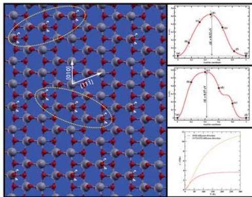
Figure 1: Water clustering onto the anatase (101) surface
