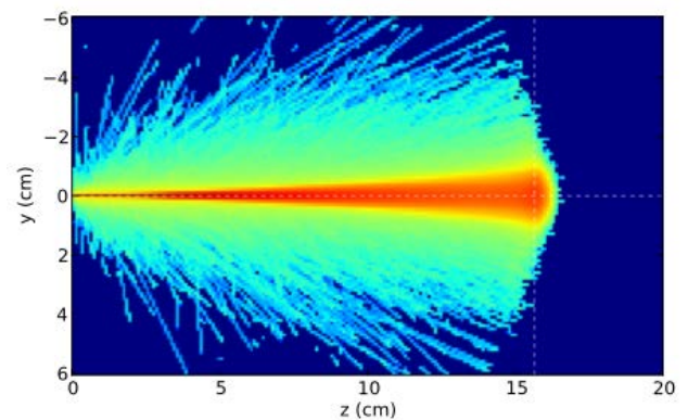
Figure 1: Dose map of a monoenergetic beam of protons in liquid water reproduced with FRED .
