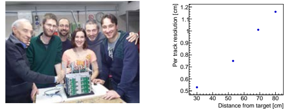
Figure 1: (Left) Final assembly of the DP detector, carried out in the SBAI department workshop of the “La Sapienza” University. The ‘naked’ detector is shown, with the readout boards (in green) and the aluminum inserts used to cool the readout circuits. (Right) Back tracking resolution obtained at different distances from the target.
