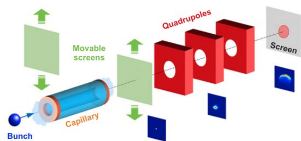
Figure 2: Focusing of High-Brightness Electron Beams with Active-Plasma Lenses: experimental layout [1].
