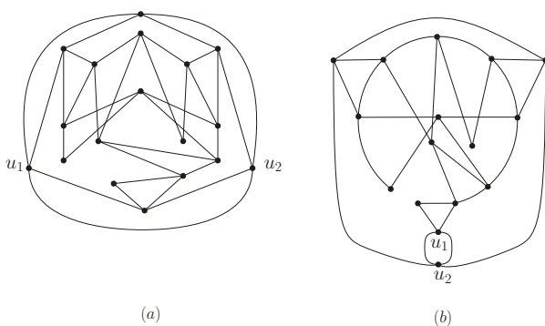
Figure 1: Fiol's and Chetwynd's critical graphs
