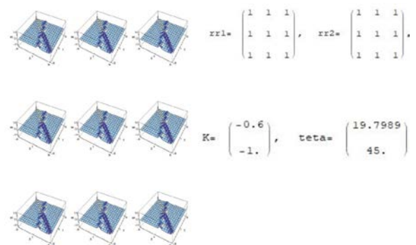
Figure 1: Solution of a 3x3 matrix mKdV equation.
