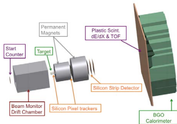
Figure 1: Schematic view of the FOOT apparatus.
