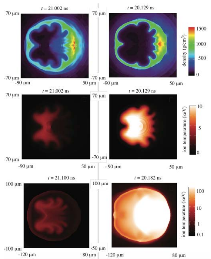
Figure 1: Simulation of shock ignition targets, driven by nonuniform laser pulses, and mispositioned. Maps of density and ion temperatures at implosion stagnation and ignition. Two targets (right and left column, respectively) are considered. Only the target with larger ITF (on the right) ignites.
