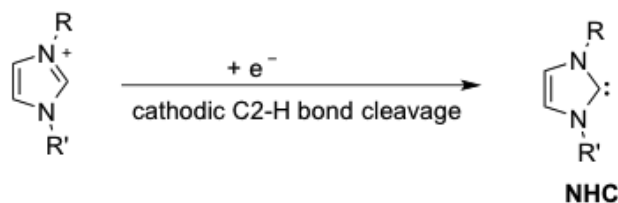
Figure 1: Electrochemical generation of NHC.
